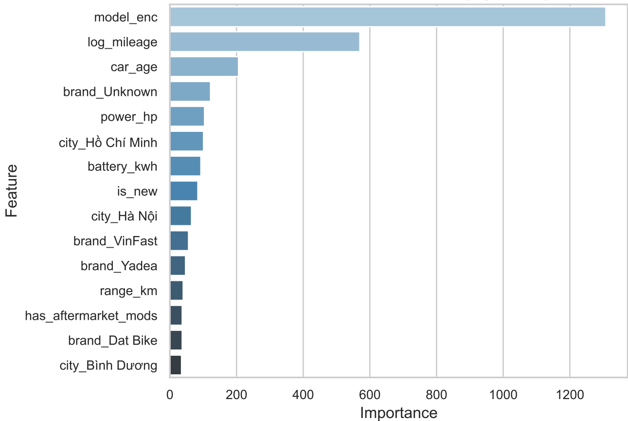
Top 15 Feature Importances (LightGBM)
