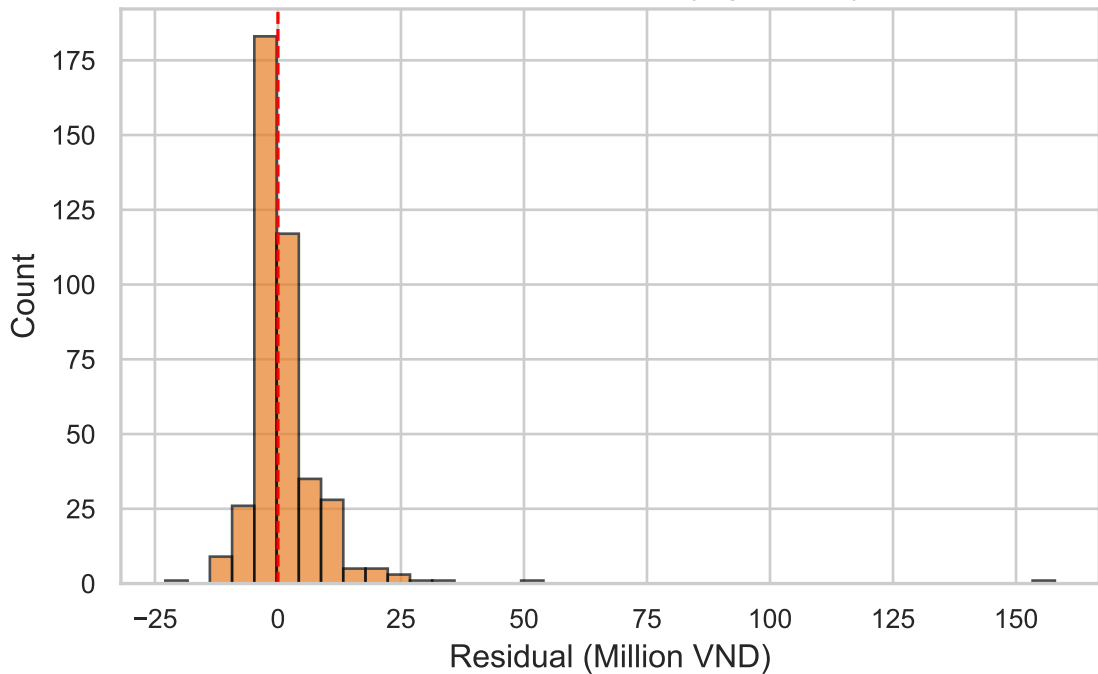
Residual Distribution (LightGBM)
