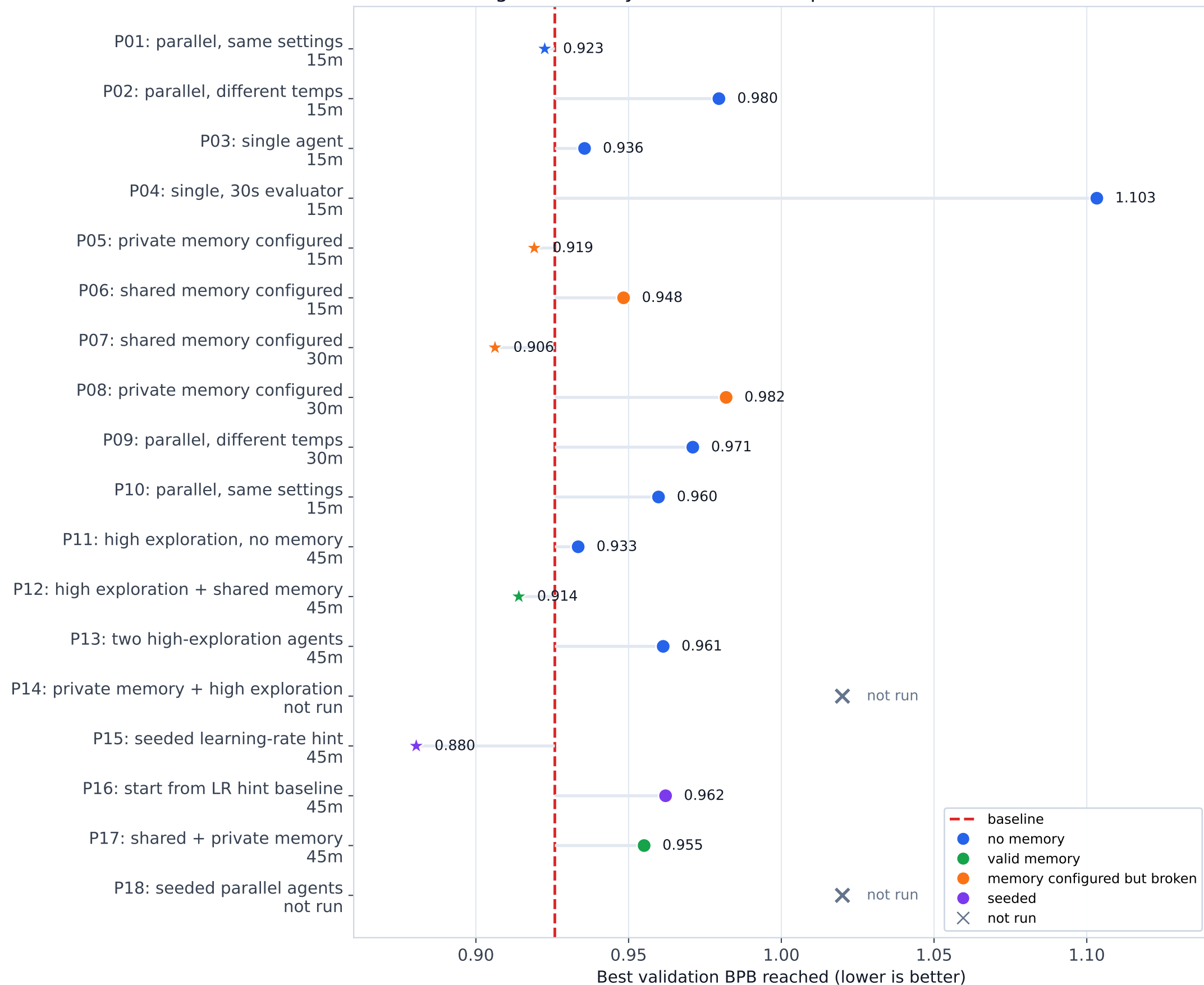
Agent memory ablation: which probes beat the baseline?
