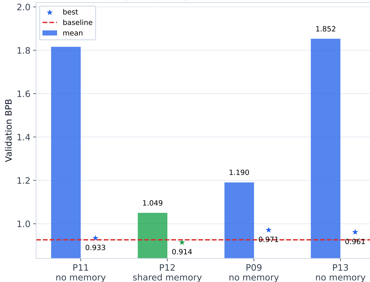
Shared memory keeps high exploration closer to baseline
