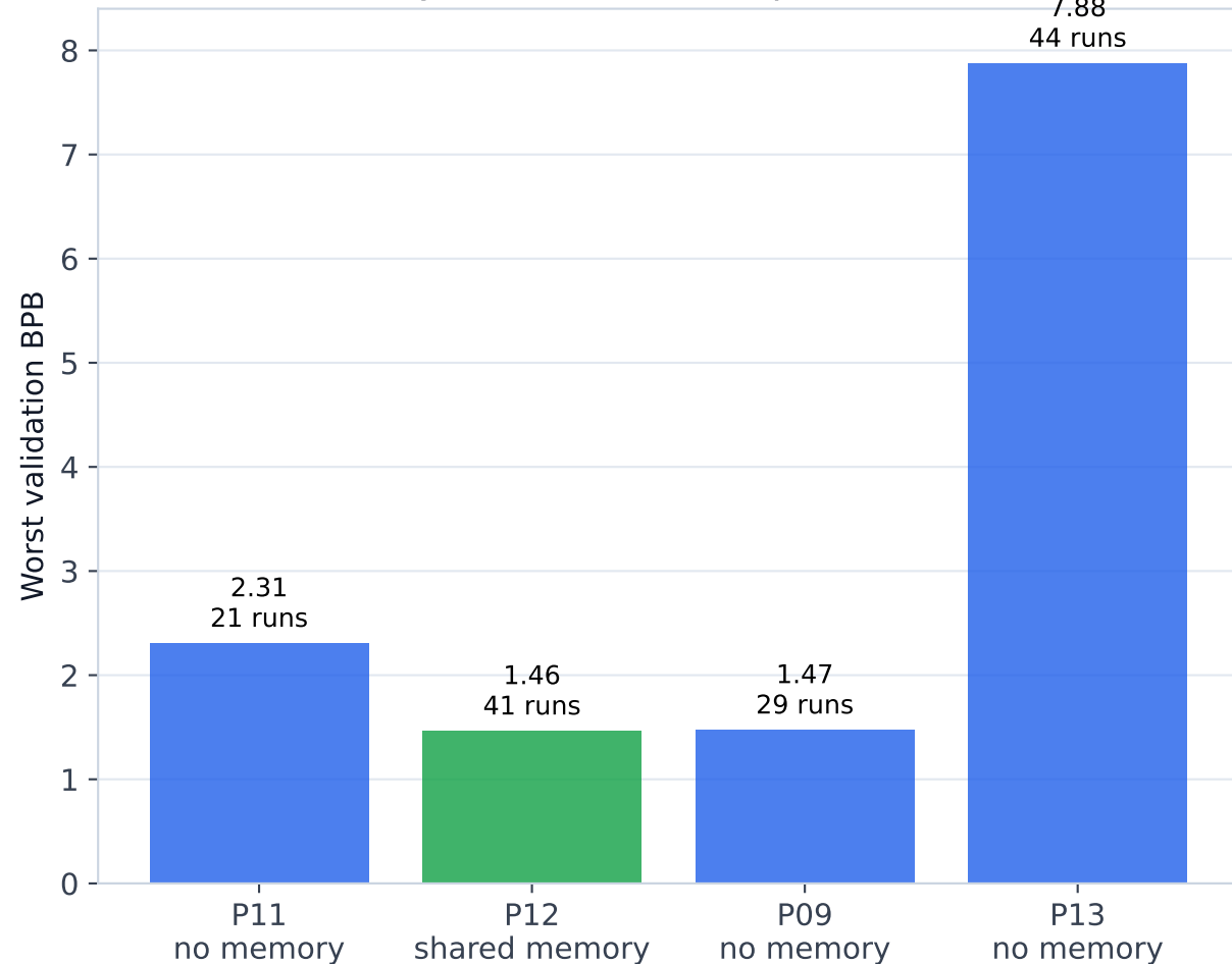
Memory reduces catastrophic outcomes
