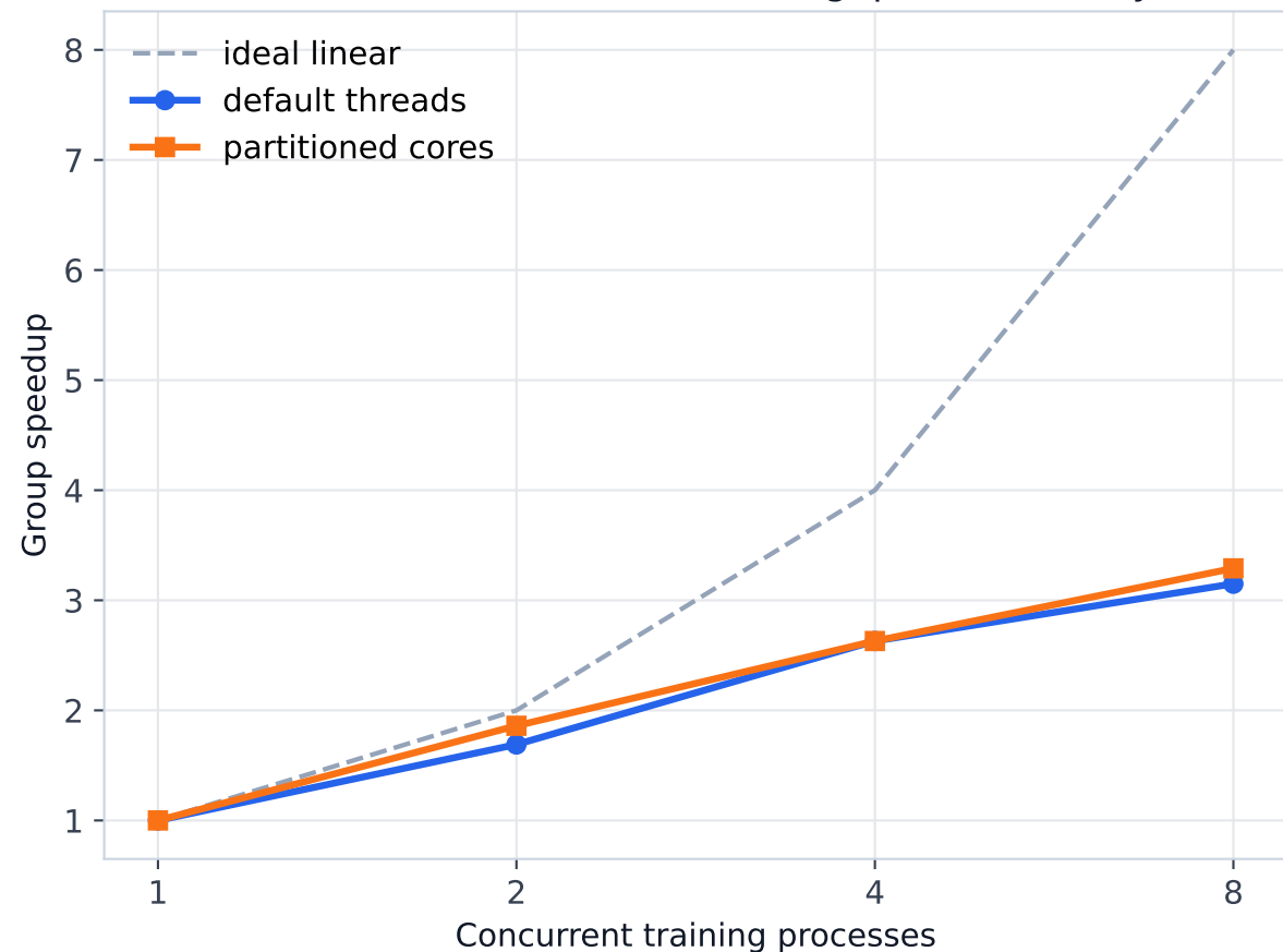
A. More workers increase throughput sublinearly
