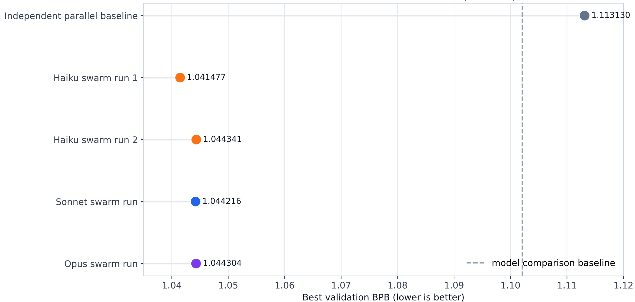
Swarm runs reached lower validation BPB than the independent-parallel baseline
