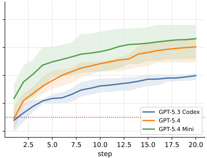
ResNet
