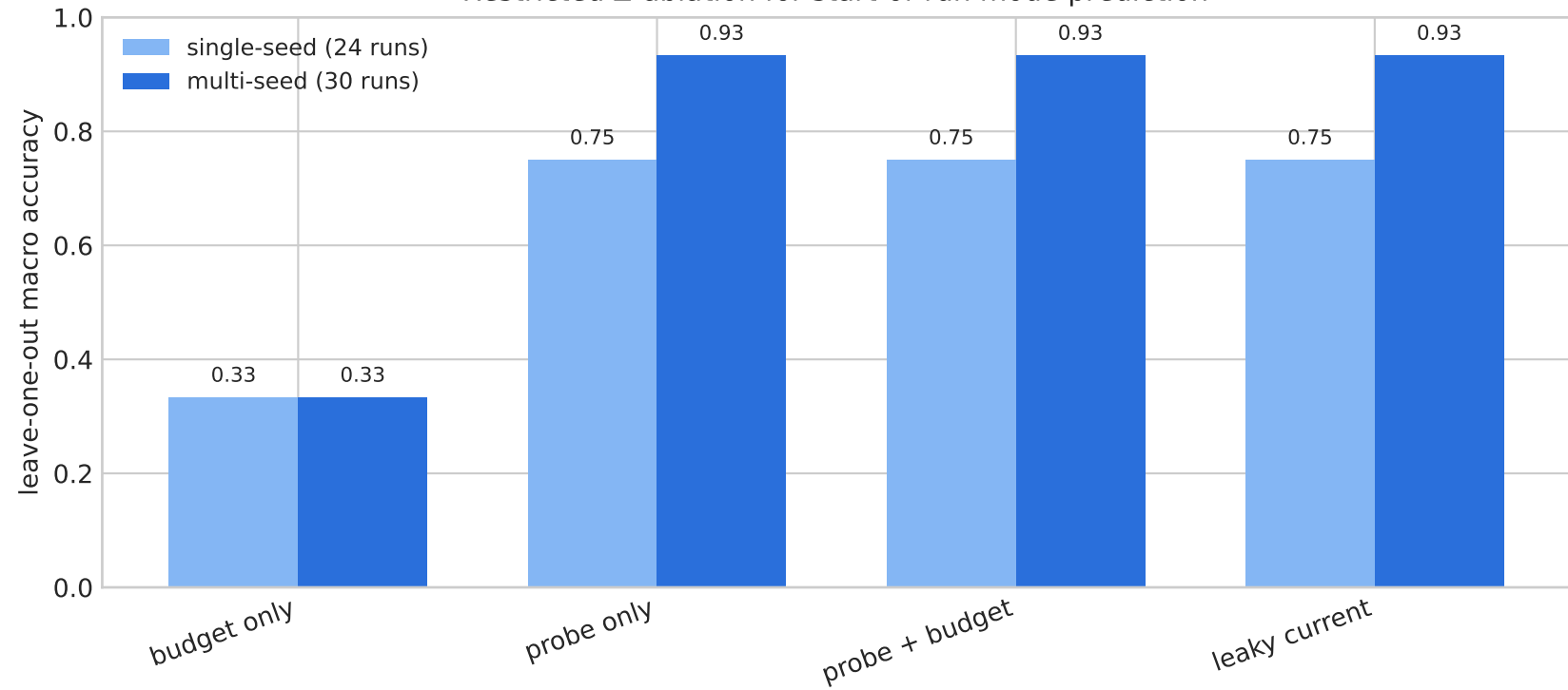
Restricted-Z ablation for start-of-run mode prediction
