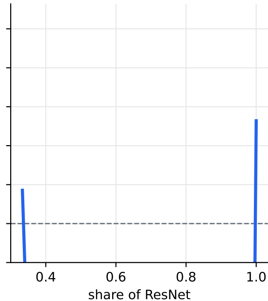
ResNet-heavy deployment
