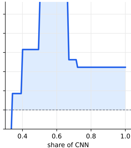
CNN-heavy deployment
