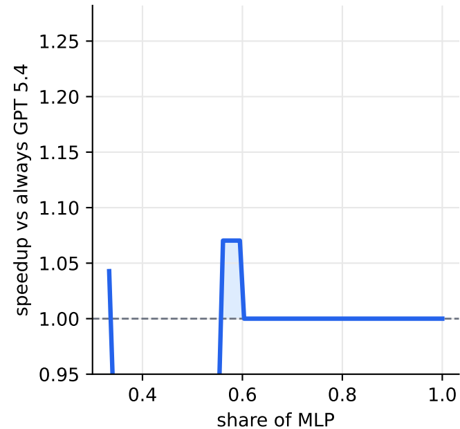
MLP-heavy deployment
