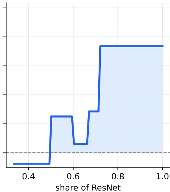
ResNet-heavy deployment
