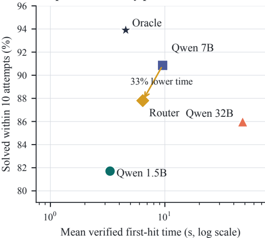
a Speed--reliability plane
