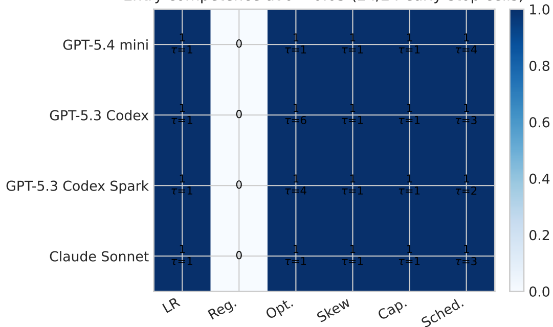
Threshold calibration from the 24-cell early-stop pilot
