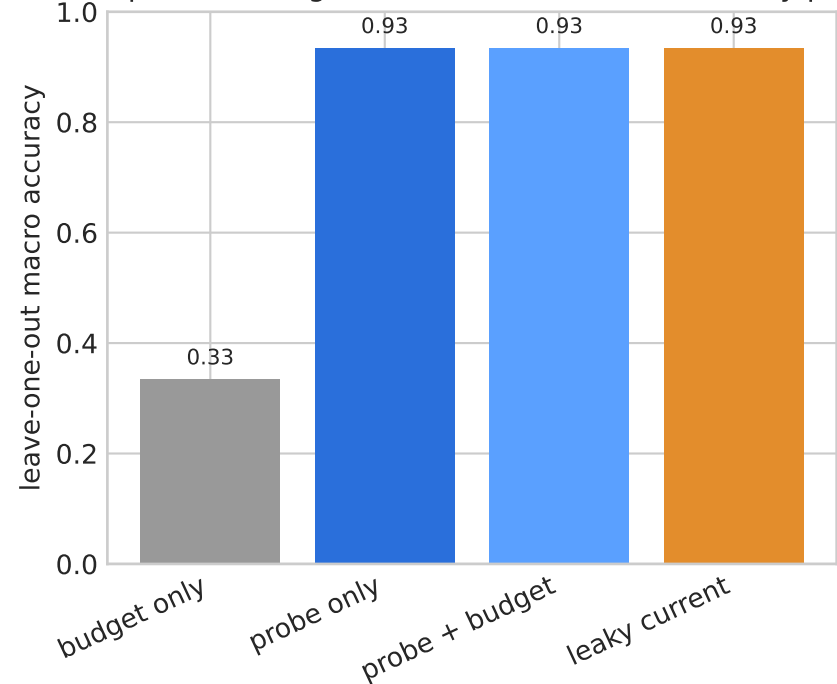
Mode-prediction signal ablation on 30 baseline-only probes
