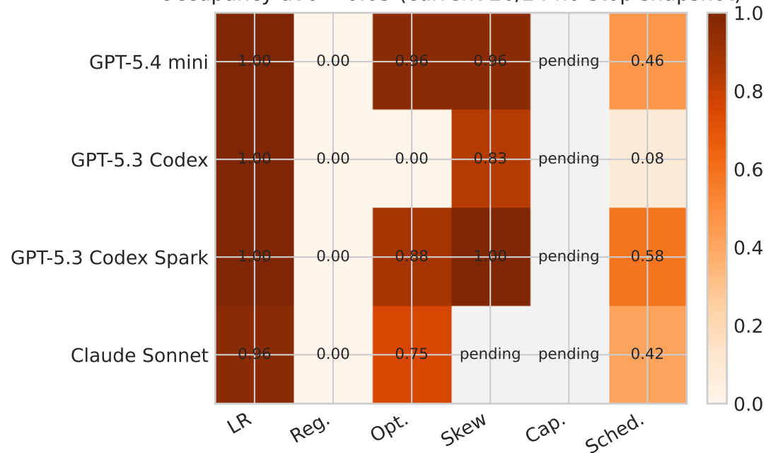
Mode-prediction signal ablation on 30 baseline-only probes
