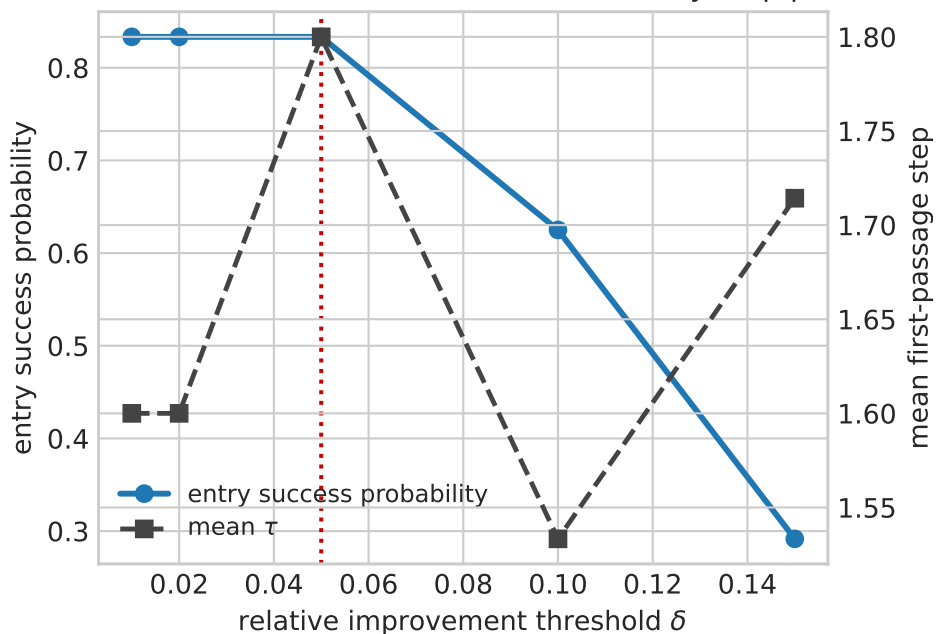
Threshold calibration from the 24-cell early-stop pilot
