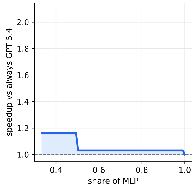
MLP-heavy deployment
