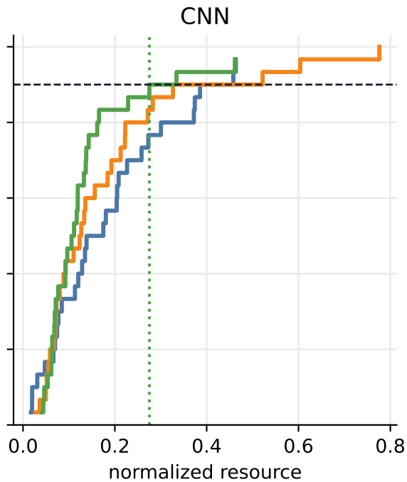
Empirical success-by-budget curves at \gamma = 0.05
