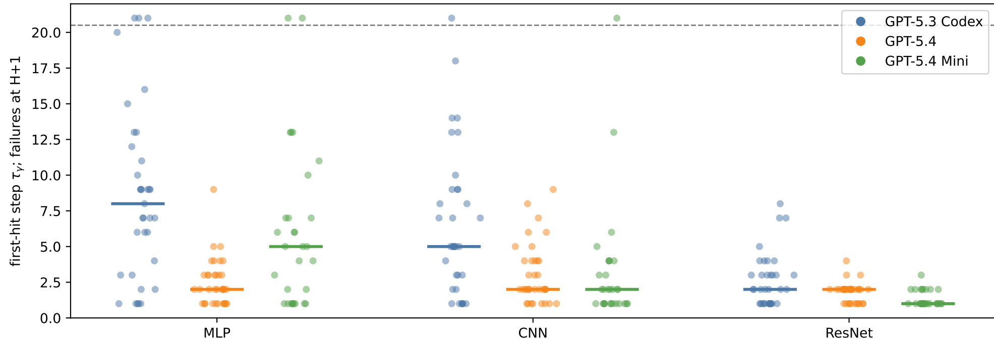
First-hit distribution
