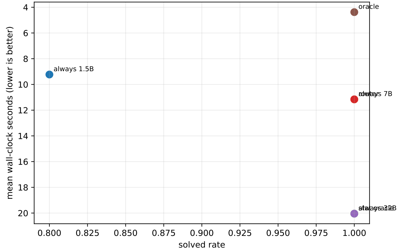
Router time vs verified accuracy
