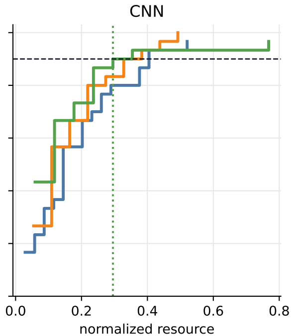
Empirical success-by-budget curves at \gamma = 0.05
