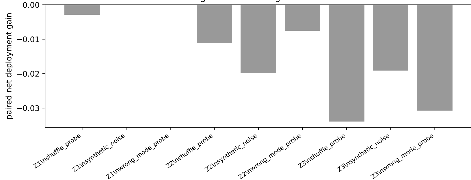
Negative-control signal checks
