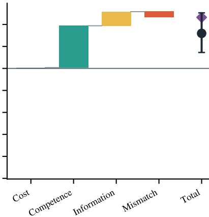
Qwen 7B
