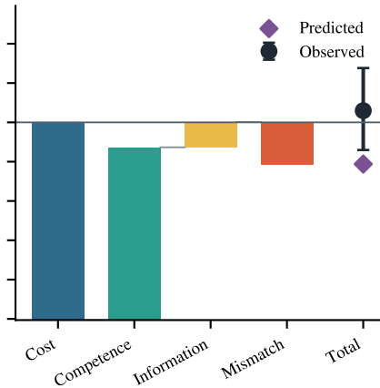
Qwen 32B
