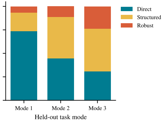
Qwen 32B
