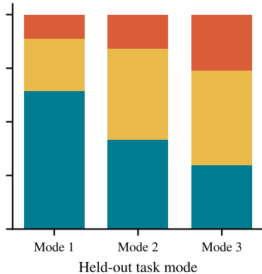
Qwen 7B
