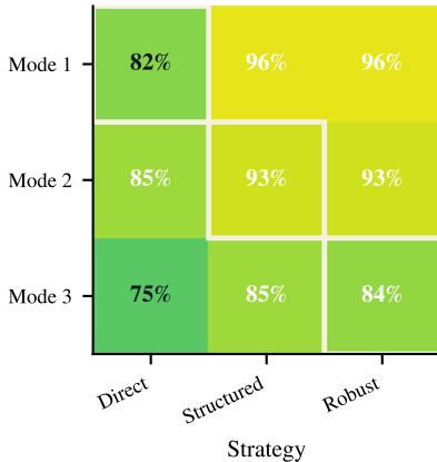
Qwen 7B
