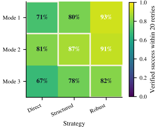
Qwen 32B
