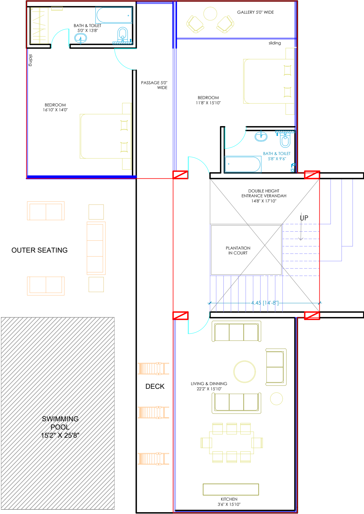
GROUND FLOOR 1648.86 SQ.FT.
