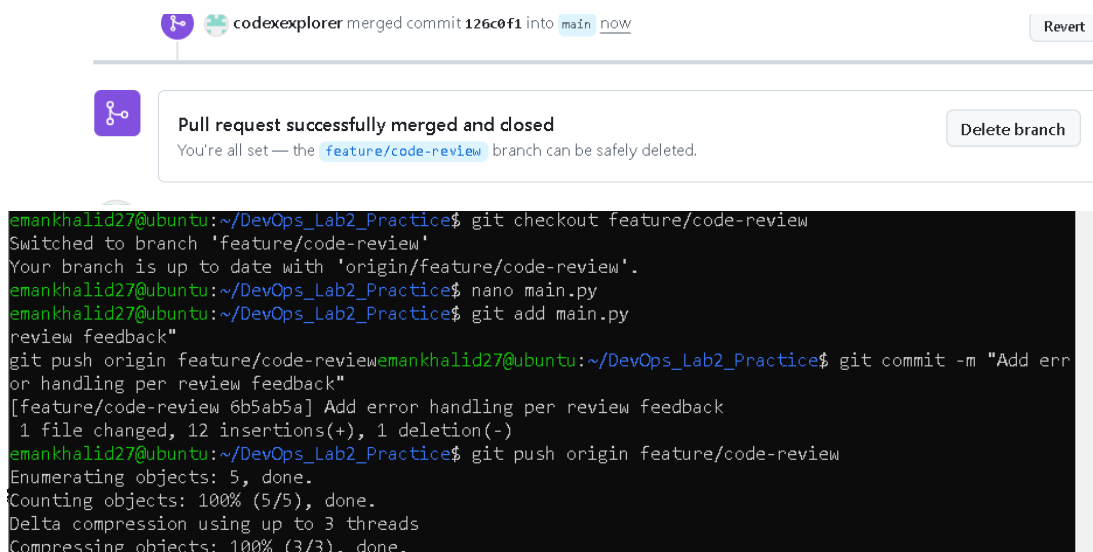
Figure 33: Merged Pull Request
