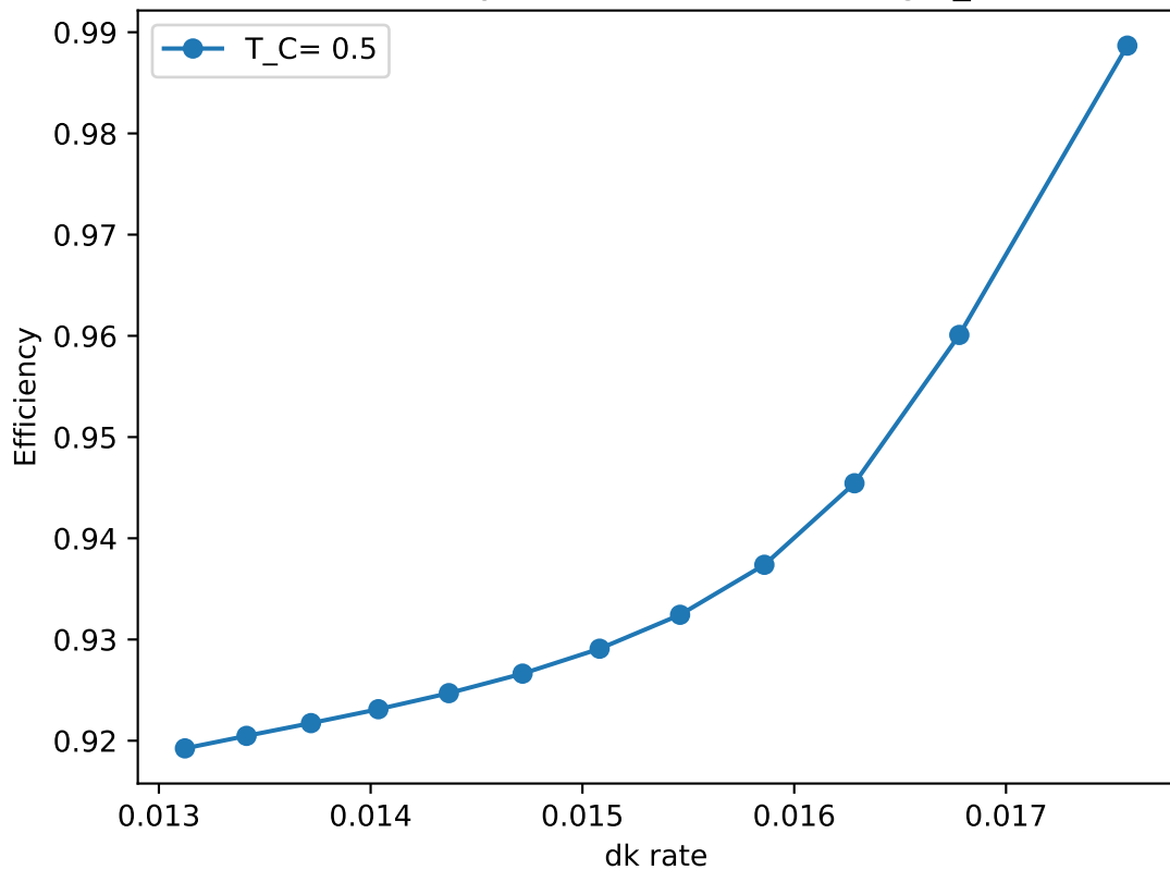
Efficiency vs dark counts , varying d_l
