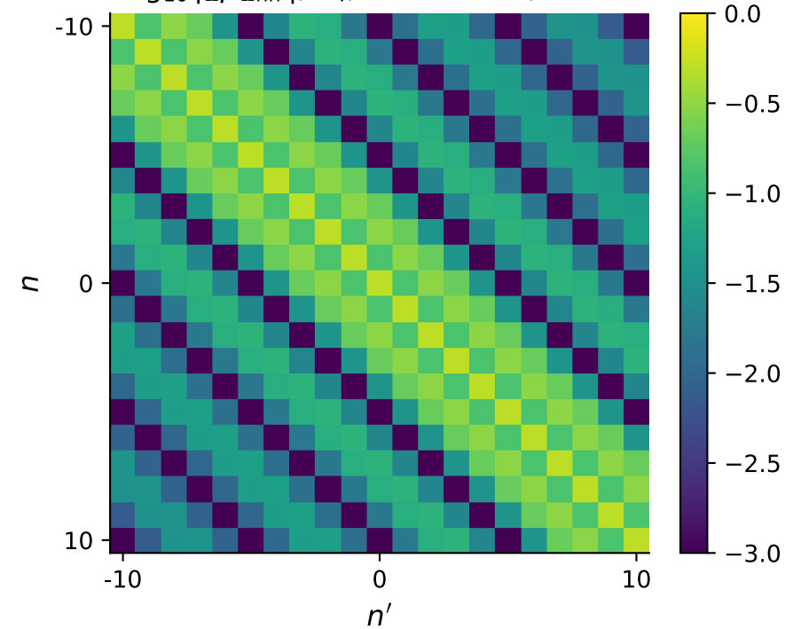
\log_{10} |[\mu]_{nn'}| , S_4 , \nu = 0.9 GHz, N = 21
