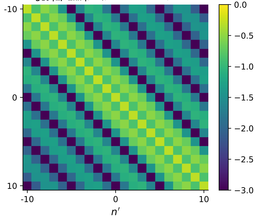
\log_{10} |[\mu]_{nn'}| , S_4 , \nu = 0.9 GHz, N = 21
