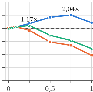
soc-Pokec
