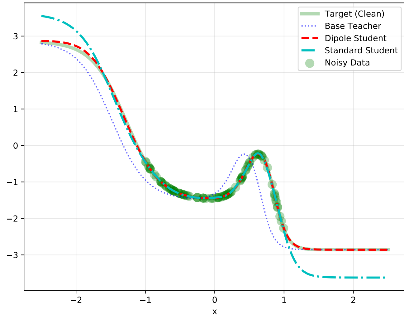
Result: Dipole vs Standard (Target shifted by \delta = 0.2 )
