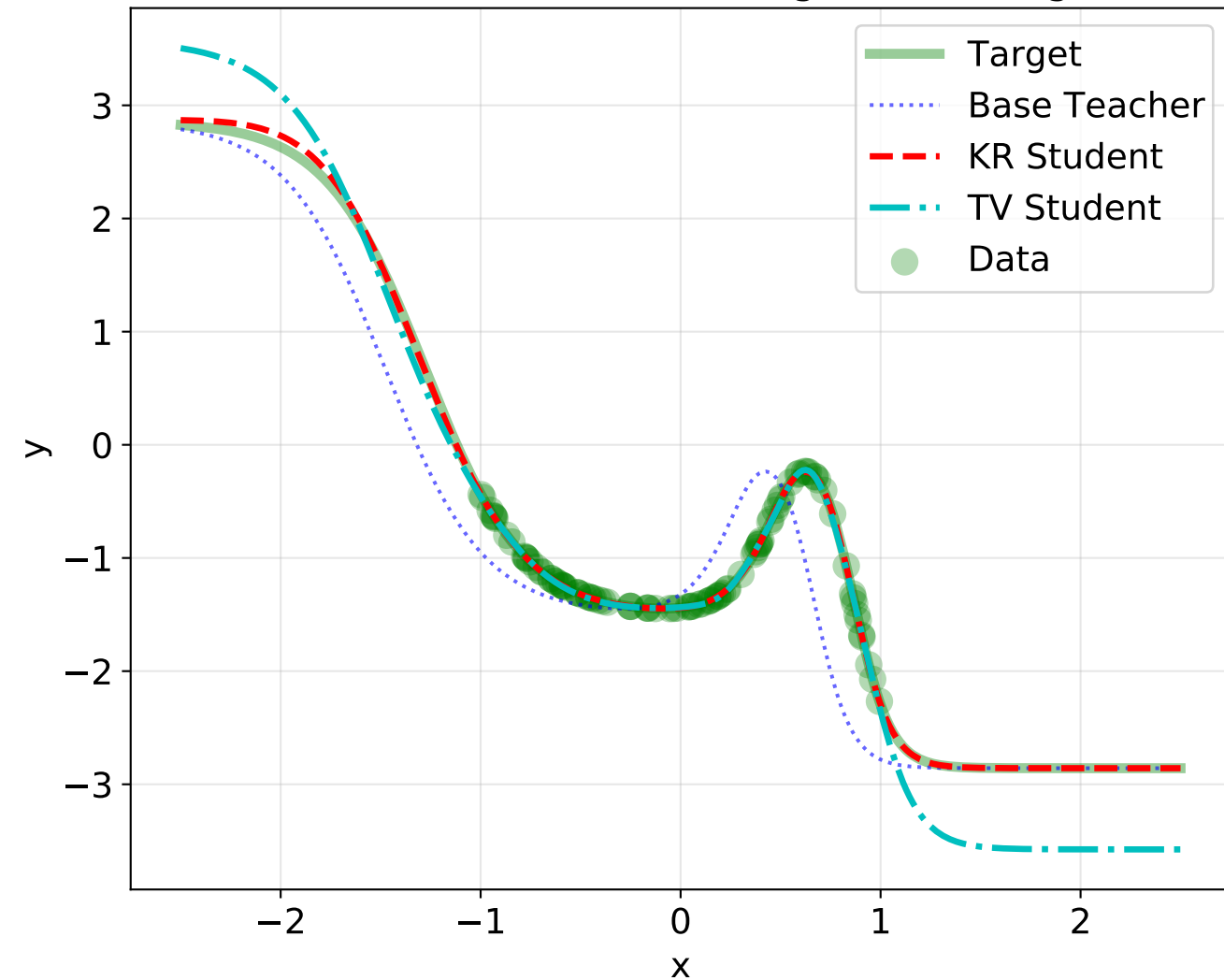
Reconstruction of the target function g
