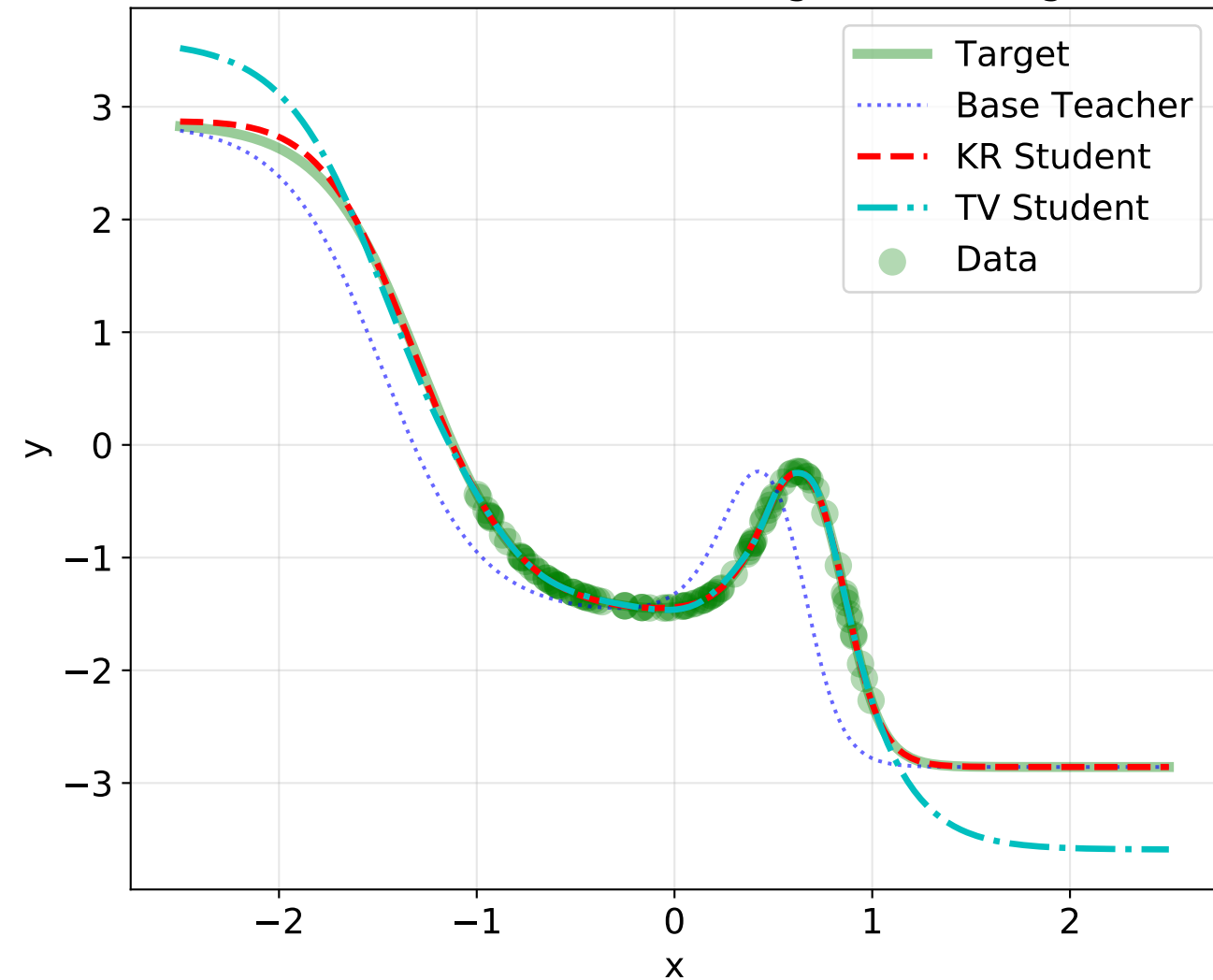
Reconstruction of the target function g
