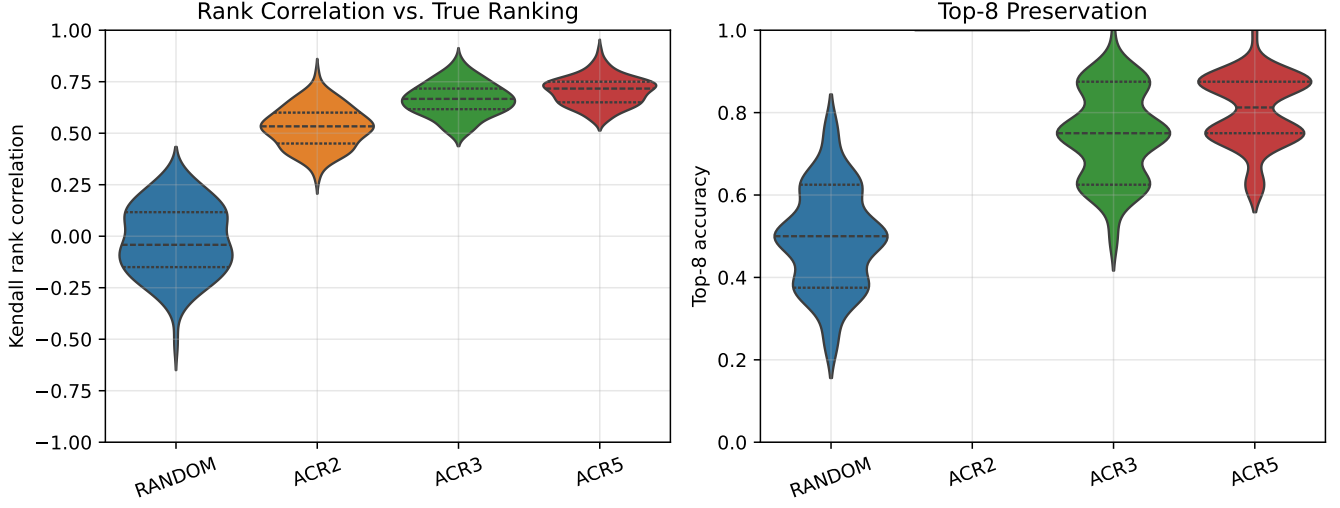
Figure 7: Seeding quality distribution across 100 variants per class. Left: Kendall rank correlation. Right: top-8 accuracy. RANDOM: complete shuffle; ACR2: top-8/bottom-8 preservation; ACR3: preserves three segments (top-4, middle-8, and bottom-4); ACR5 preserves top5; middle-6 and bottom-5. ACR2 has a top-8 preservation of 1.0 by construction.
