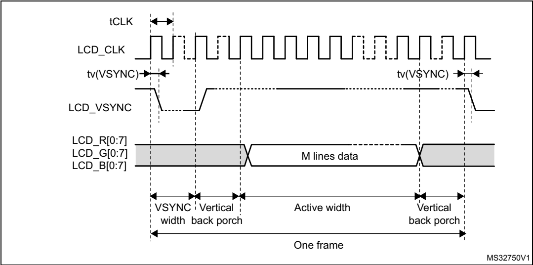
Figure 100. LCD-TFT vertical timing diagram
