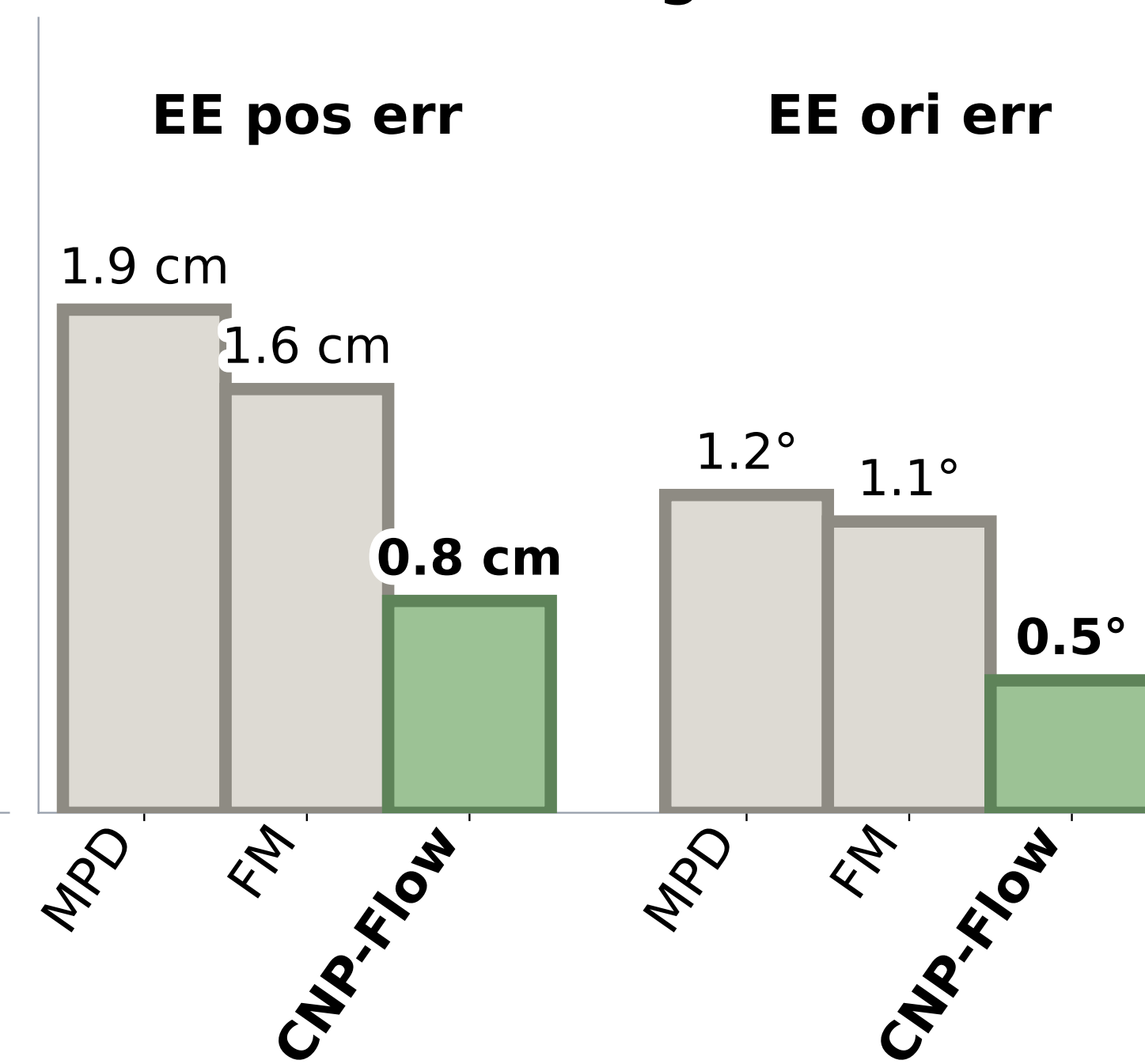
Motion Planning EE Error ↓
