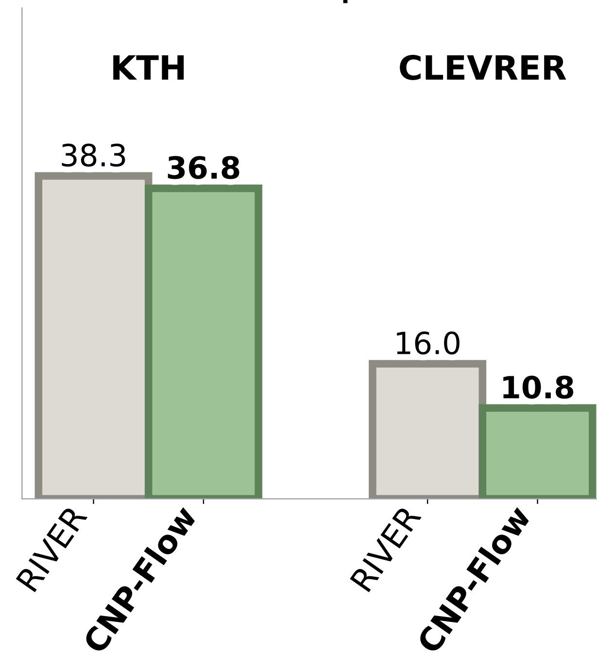
Video Interp. FVD ↓
