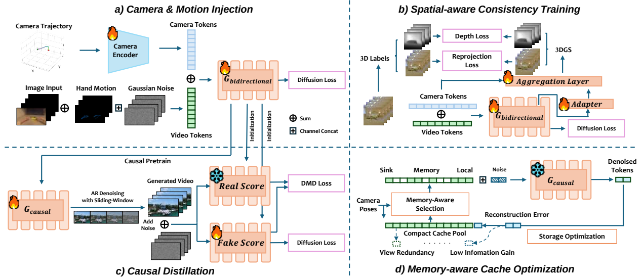
Figure 3: Framework of WorldScape. a) Given camera trajectory and pose video of hand motion, WorldScape trains a bidirectional teacher model backbone along with a camera encoder to enable controllable video generation. b) In Spatial-aware Consistency Training, WorldScape trains a feature aggregator together with an adaptor that projects DiT latents into the input space of the aggregator. The aggregator predicts depth and 3D information to compute two consistency losses, thereby training the model to maintain 3D consistency during video generation. c) WorldScape employs a Self Forcing-style distillation to transfer the controllability and spatial consistency of the bidirectional teacher DiT into an autoregressive few-step student model. d) During inference, WorldScape maintains the KV cache based on camera poses and information gain, enabling autoregressive generation with long-horizon memory.
