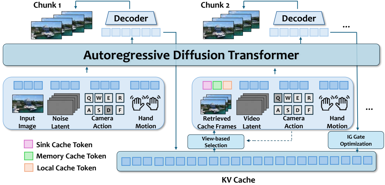
Figure 2: Model overview. WorldScape adopts a chunk-level autoregressive video generation architecture, where the denoising process of each chunk is conditioned on the camera pose inputs, hand motion inputs, and the KV cache of past denoising results.
