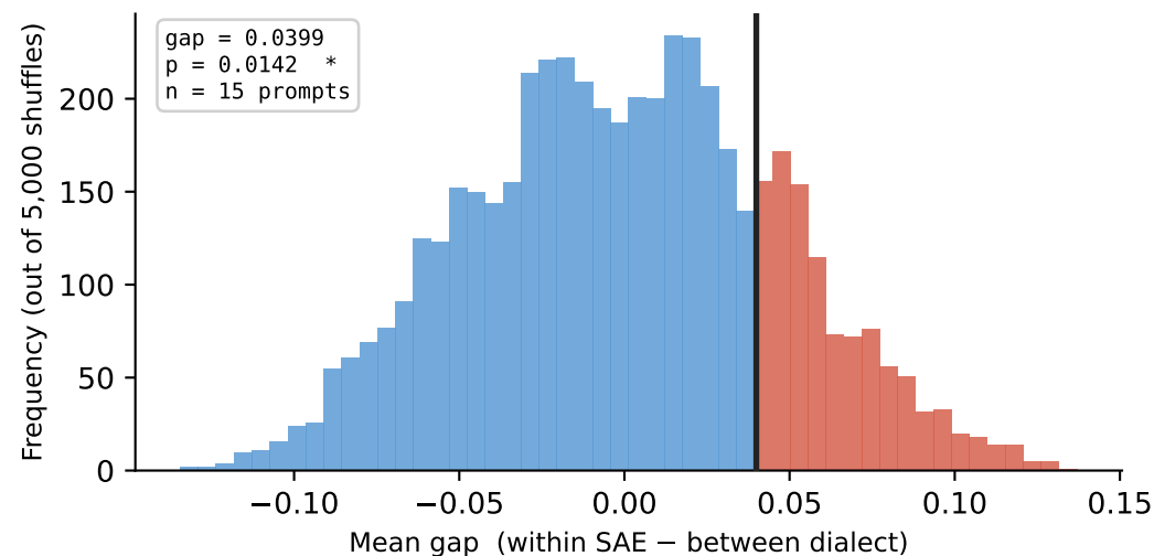
Round 1 — Bigram J
