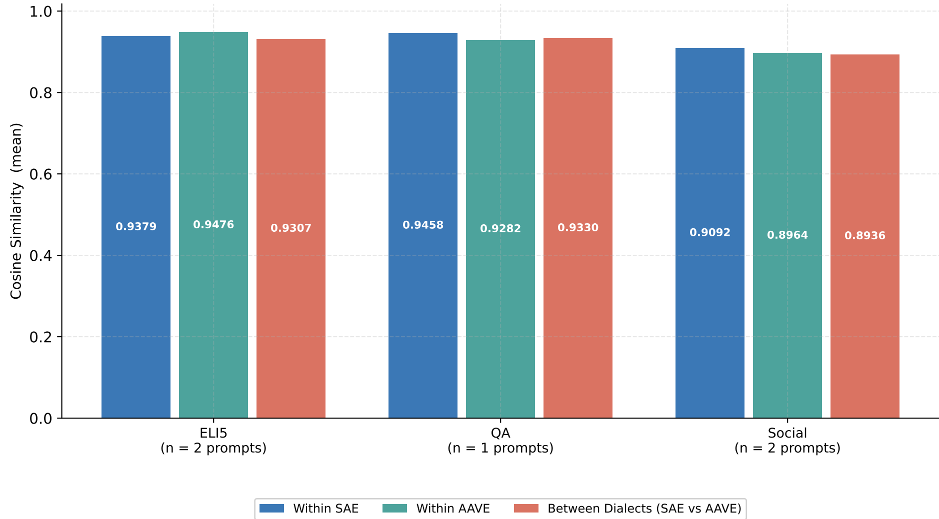
Round 2 — Per-Category Semantic Similarity (Cosine)
