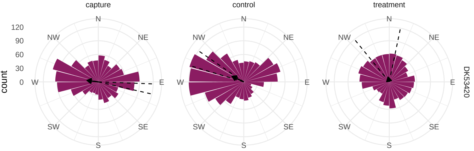
Circular Plot for Pied_Flycatcher
