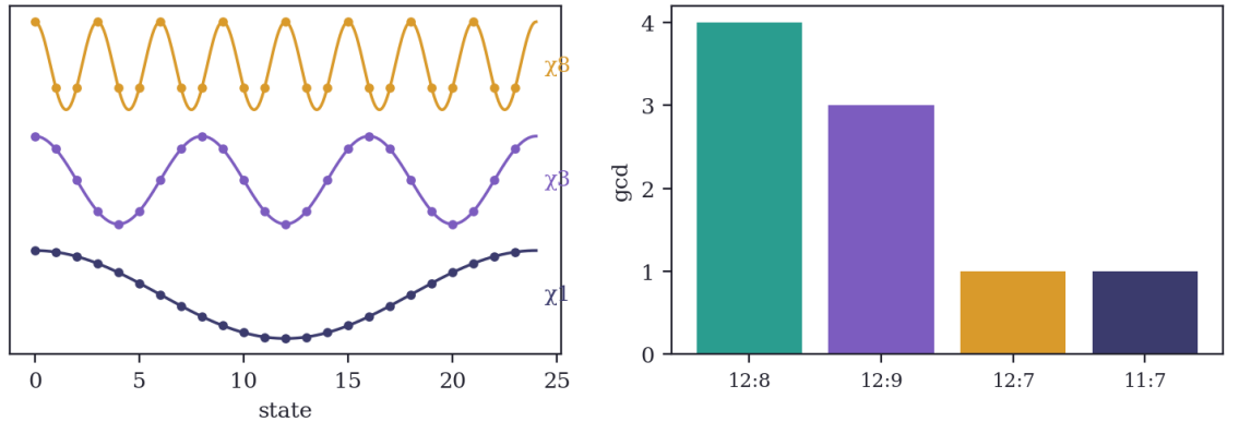
Fig. 3 — T3. Left: three characters of Z/24 . Right: consonance of frame pairs measured by gcd; the 11:7 pair shares only the trivial mode.
