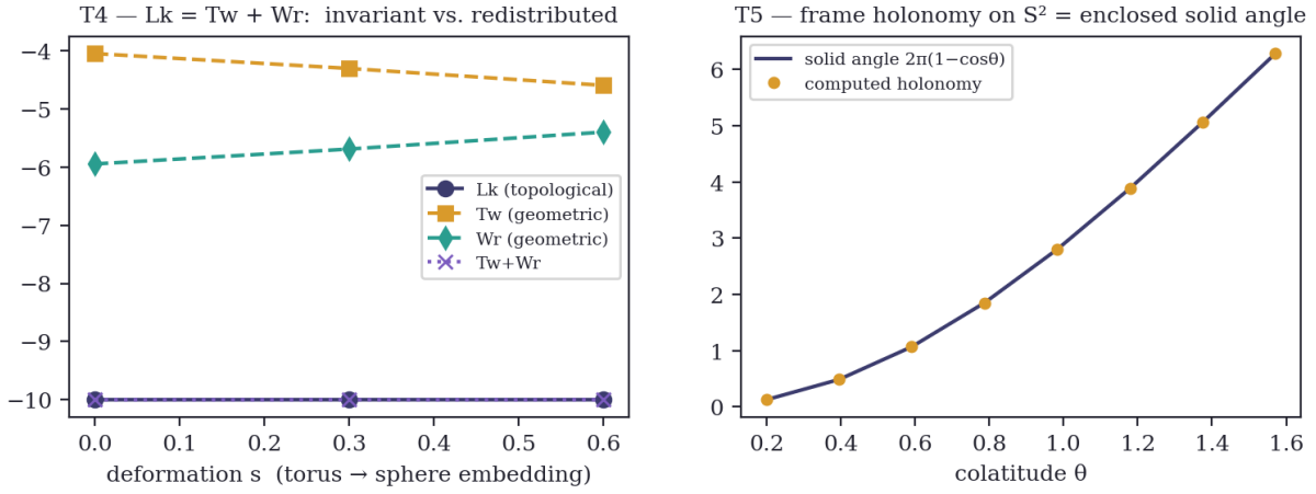
Fig. 4 — T4/T5. Left: Lk pinned at -10 across the torus→sphere deformation while Tw and Wr exchange. Right: computed holonomy vs. predicted solid angle.
