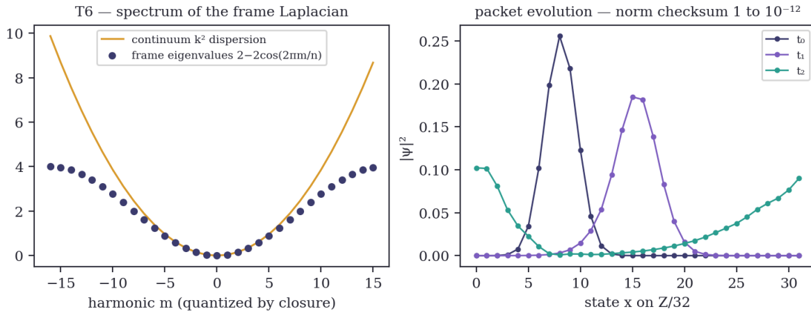
Fig. 5 — T6. Left: frame Laplacian spectrum vs. the continuum k^2 dispersion; the integer axis is quantization by closure. Right: unitary packet evolution on Z/32 with norm checksum pinned at 1 to 10^{-12} .
