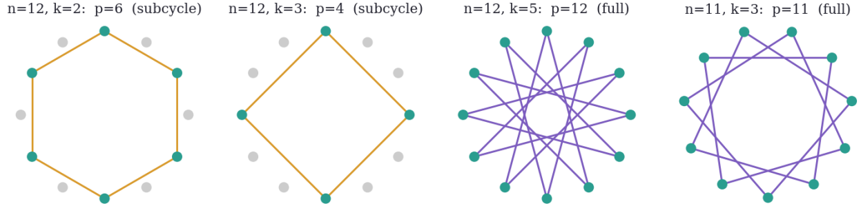
Fig. 1 — T1. Orbits of step k in Z/12 and Z/11 . Composite modulus admits early closure (subcycles, amber); prime modulus is a single full traversal for every step.
