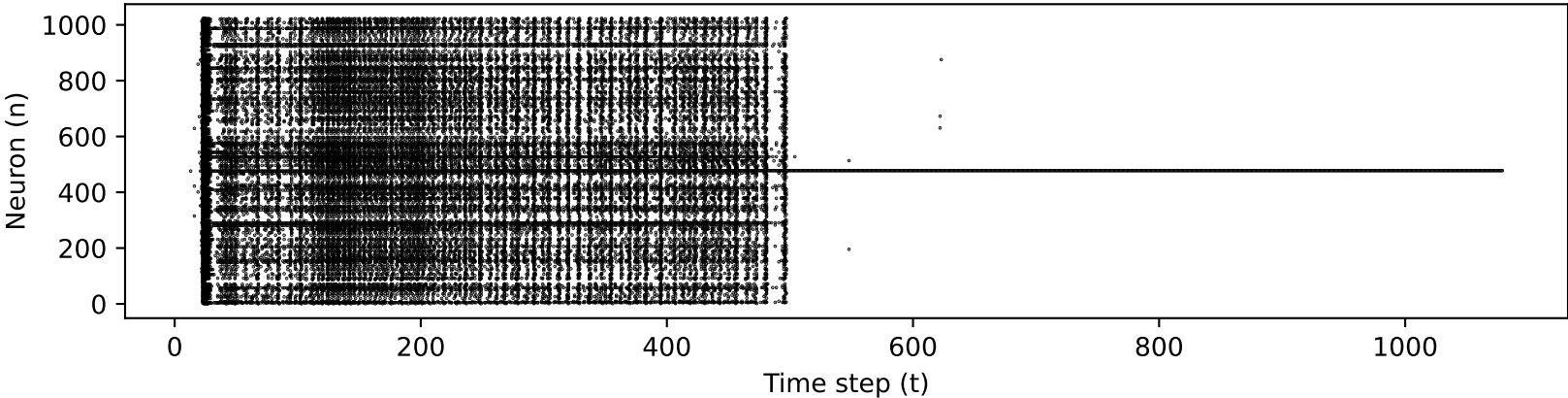
spikes_out (mean rate = 0.2543827611395179)
