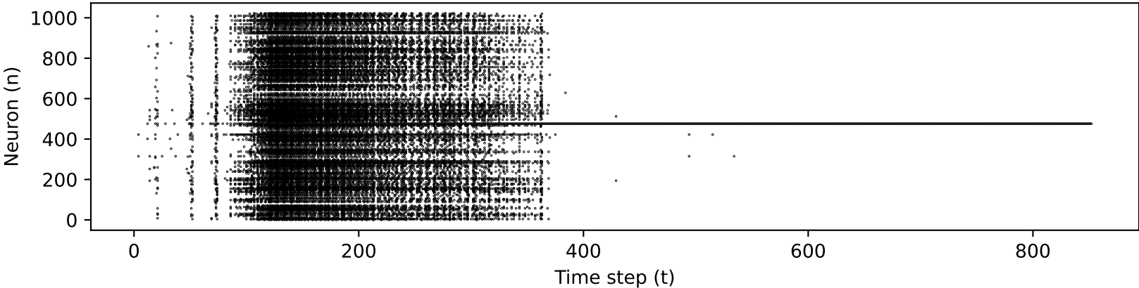
spikes_out (mean rate = 0.17388604821037254)
