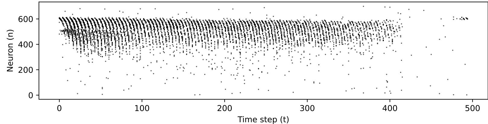
spikes_hidden_0 (mean rate = 0.02125467951059167)
