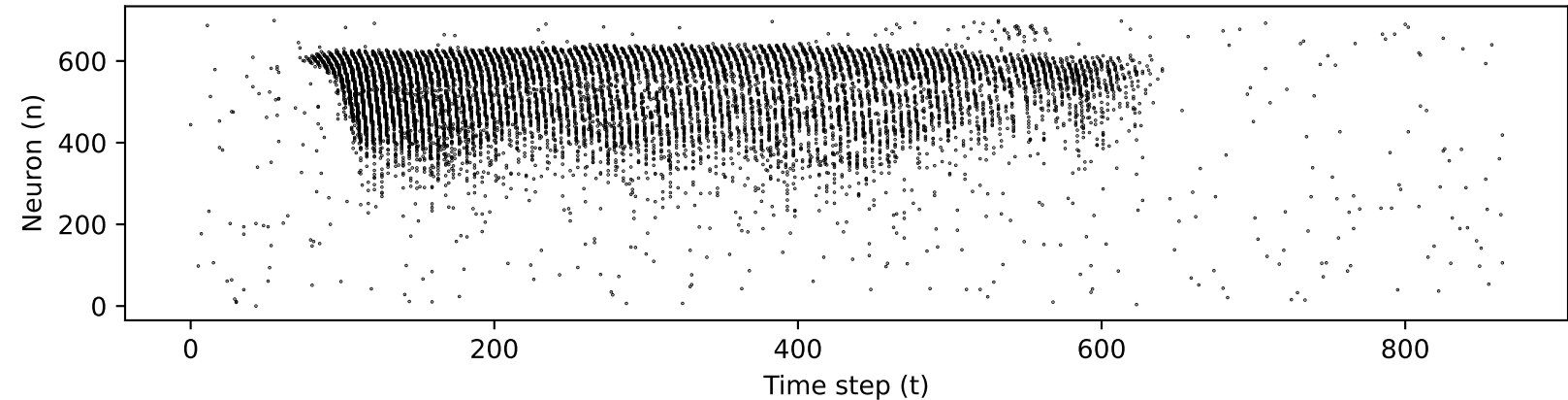
spikes_hidden_0 (mean rate = 0.0316994042184076)
