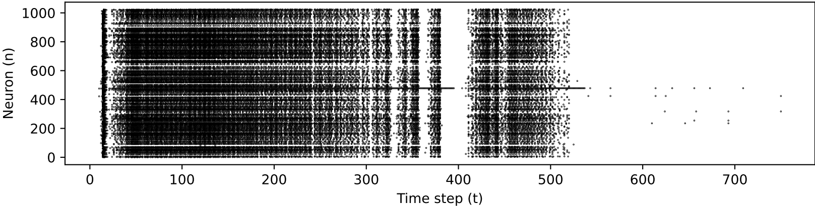
spikes_out (mean rate = 0.3028853177501826)
