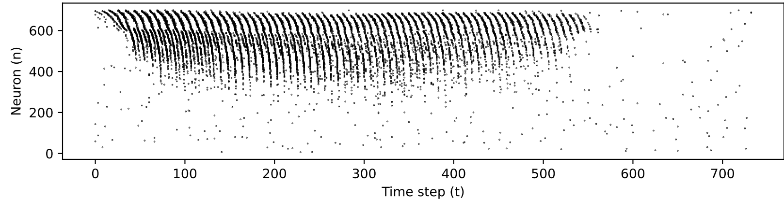
spikes_hidden_0 (mean rate = 0.028411620023739956)
