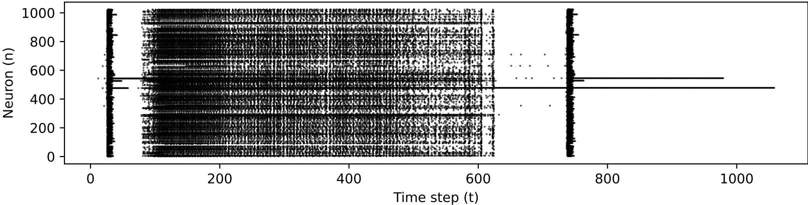
spikes_out (mean rate = 0.25613586559532503)
