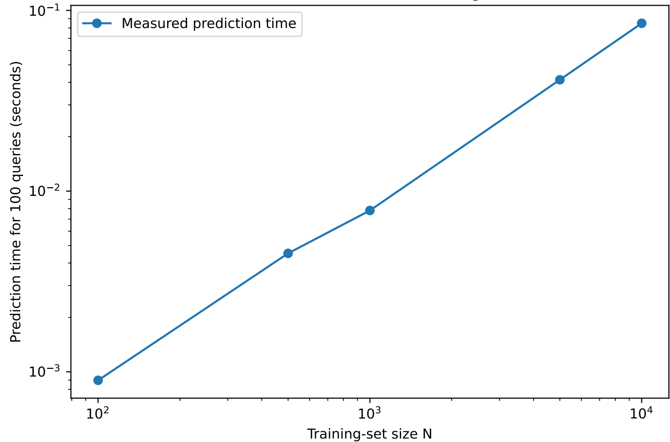
KNN Prediction Runtime vs. Training-Set Size
