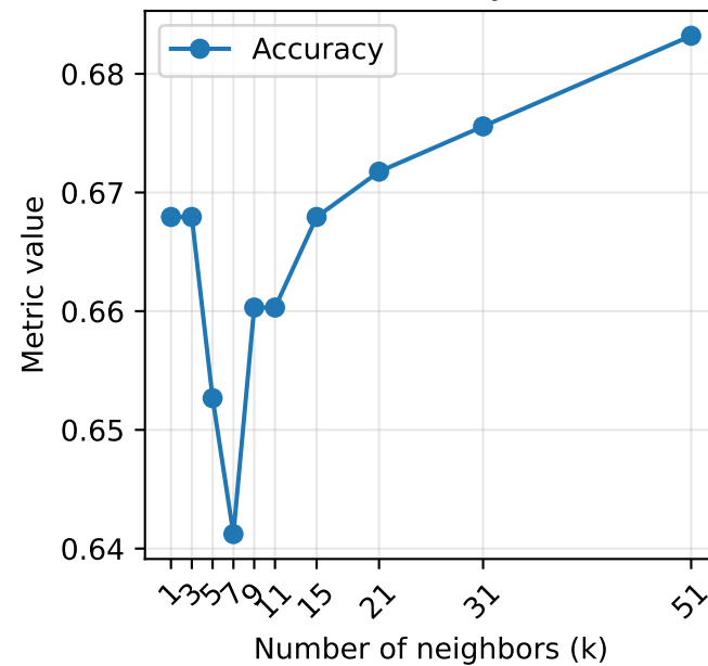
Accuracy
