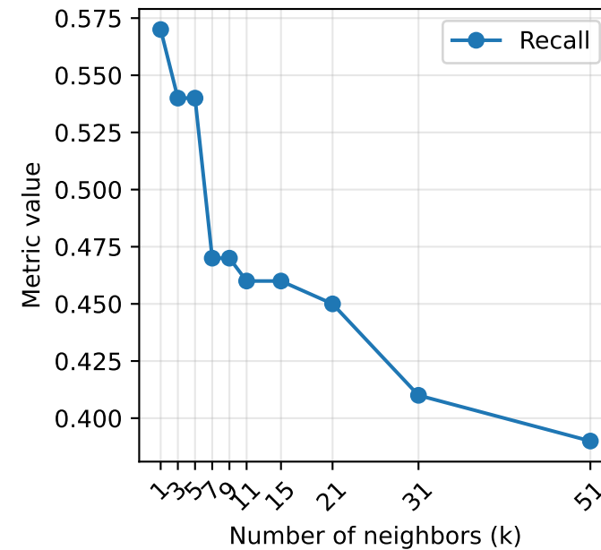
Recall
