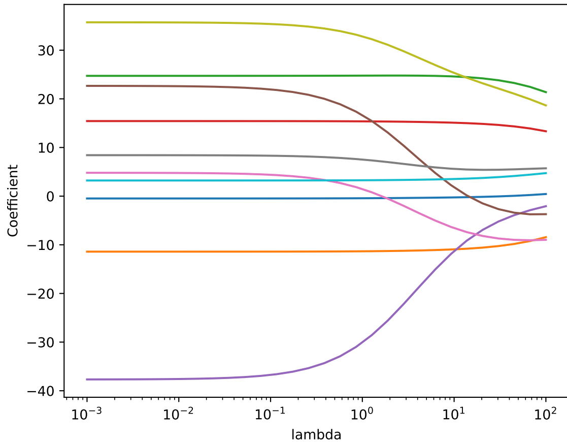
Ridge coefficient path
