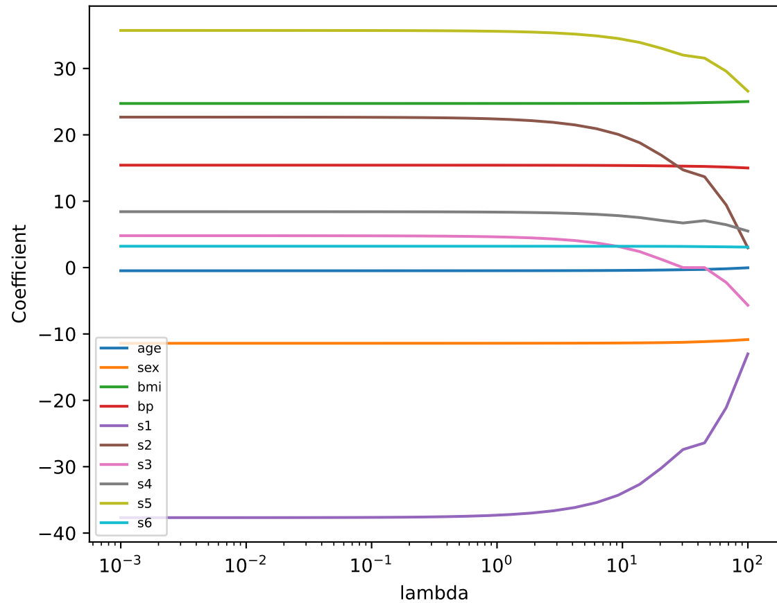
Lasso coefficient path
