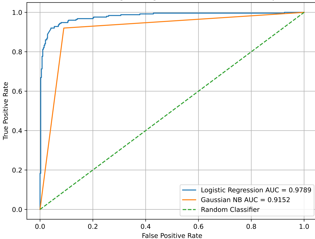
ROC Curves: Logistic Regression vs Gaussian Naive Bayes
