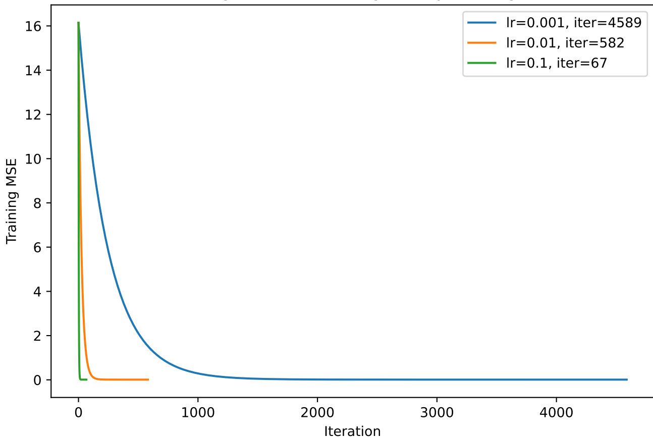
LinearRegressionGD training MSE by learning rate
