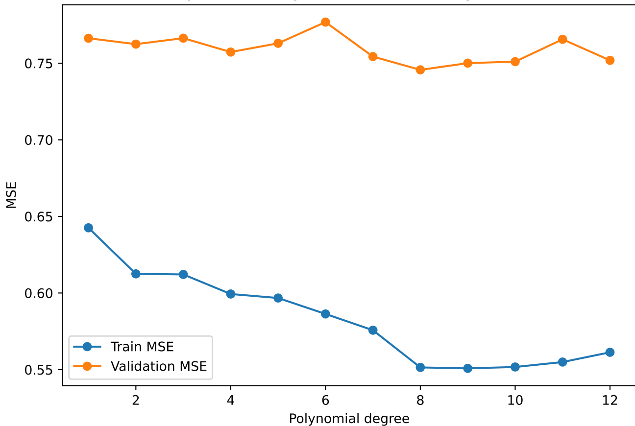
Polynomial fitting on California Housing MedInc
