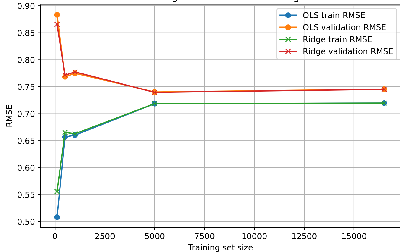
Learning Curves for OLS and Ridge
