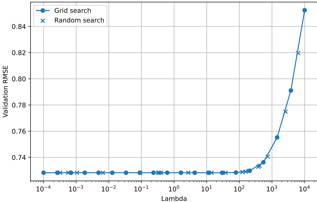
Ridge Hyperparameter Search on California Housing
