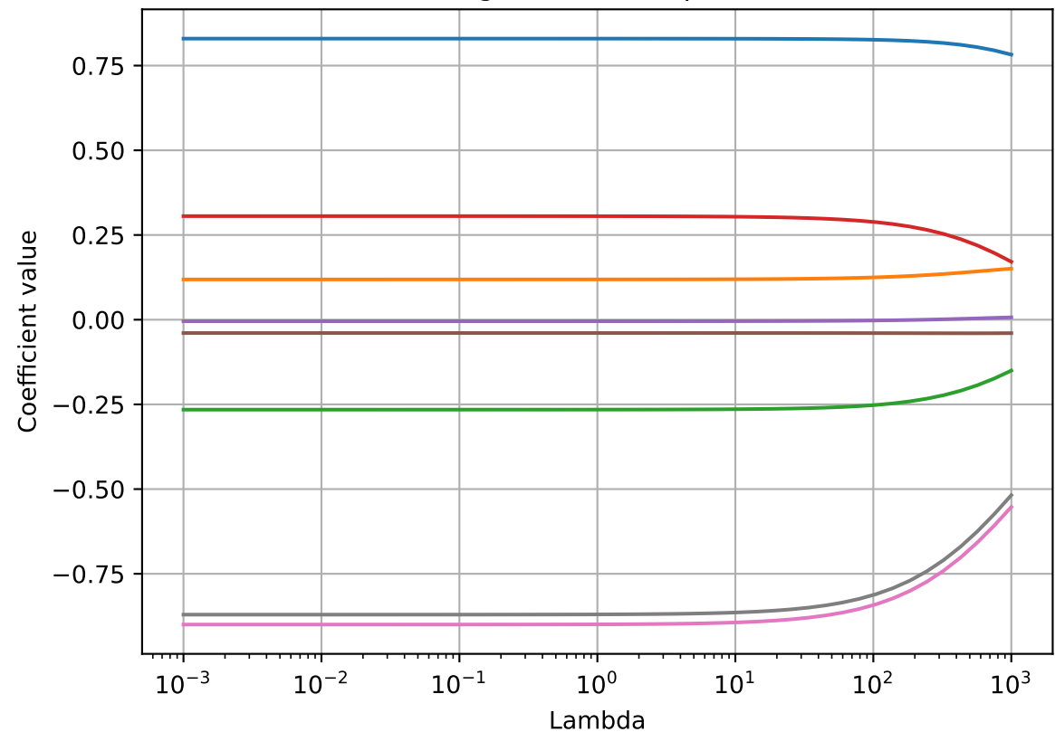
Ridge coefficient paths
