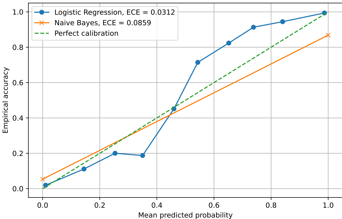
Calibration Curve for Text Classification
