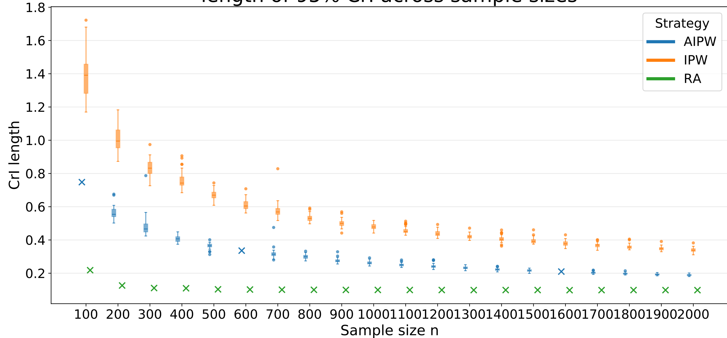
length of 95% Crl across sample sizes
