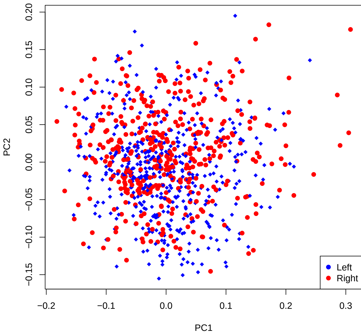
PCA of Shape by Chirality
