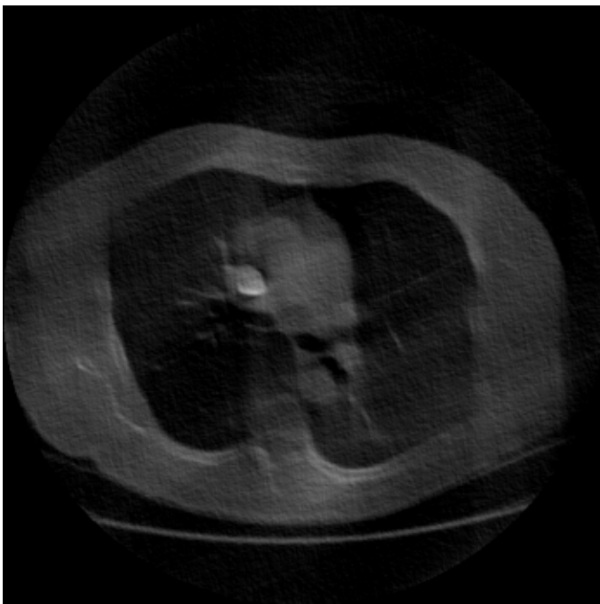
40° range, 360 projections
