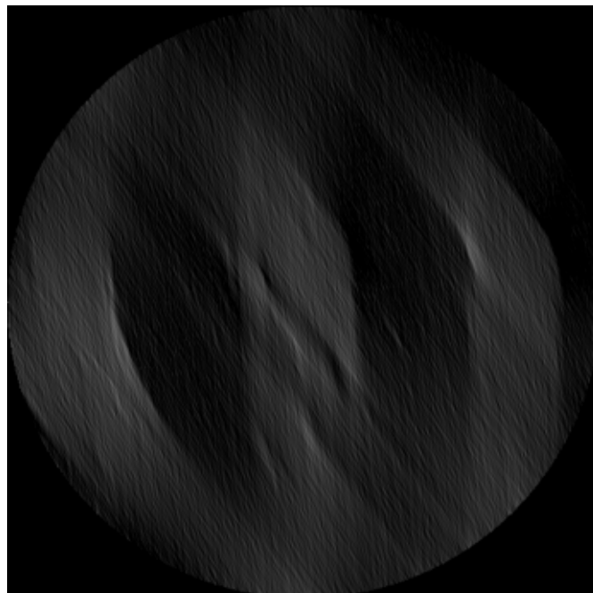
40° range, 90 projections
