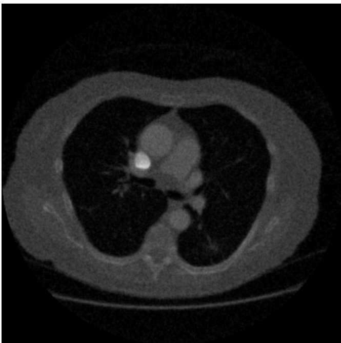
120° range, 360 projections
